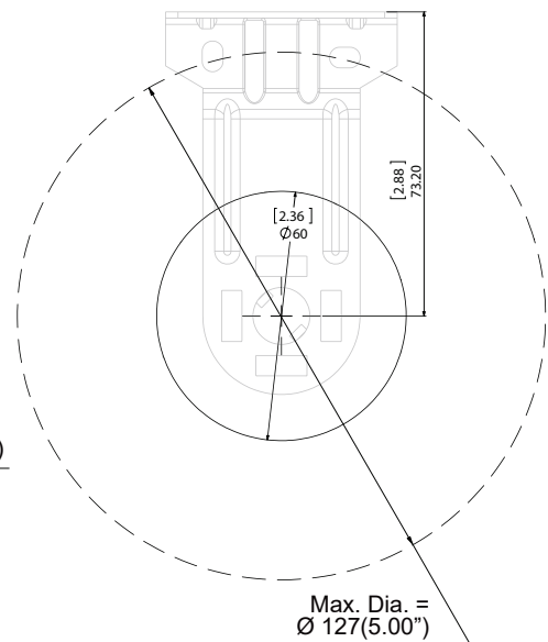
XL-F51 XL Clutch Bracket 2 7/8" Projection
