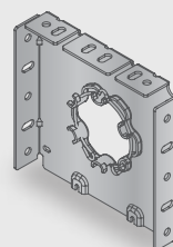
RS-37* 5.5" Star Head L Fascia Bracket with Spring Ring
