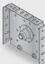
RS-39*/RS-49* 5.5" L Fascia Bracket with Single 12mm/10mm Swivel Ball Bearing
