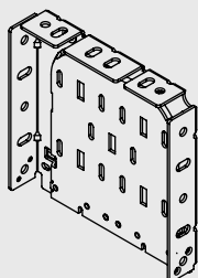
comming soon RS-D8* 5.5" L Fascia 1 1/2" RS Clutch Bracket
