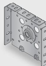
RS-38* 5.5" Intermediate L Fascia Bracket with Single 12mm Bearing
