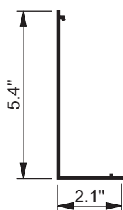
No Fascia Notching for Single Shade
