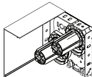
Flip Fascia for Duo Shade
