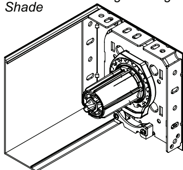
No Fascia Notching for Single Shade
