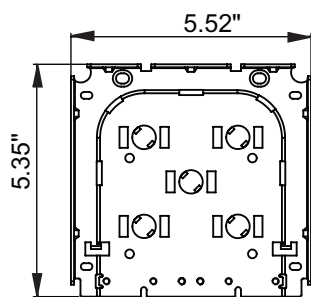
No Fascia Notching for Single Shade
