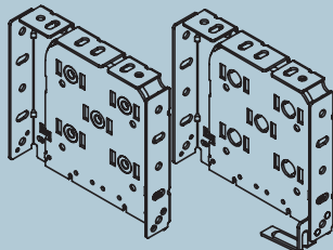
XL-E8*/XL-E9* 5.5" L Fascia XL Bracket with Clip Right/Left
