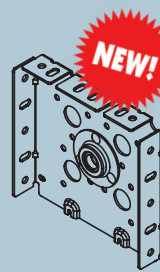
RS-38* 5.5" Intermediate L Fascia Bracket with Single 12mm Bearing
