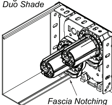
Regular Installed Fascia for Duo Shade
