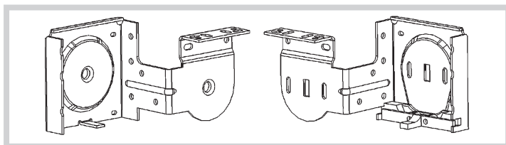
Enhanced blackout duo shade fascia bracket for 1-1/2" RS Clutch
