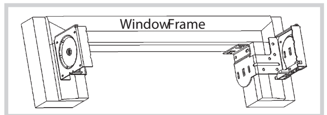
Enhanced blackout duo shade fascia bracket for 1-1/2" RS Clutch
