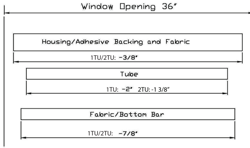
When using ST-A01 Bracket
