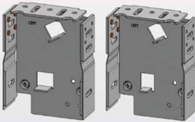
Control Side Bracket
